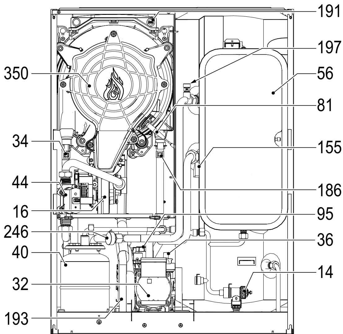
fig. 60- Vista general
