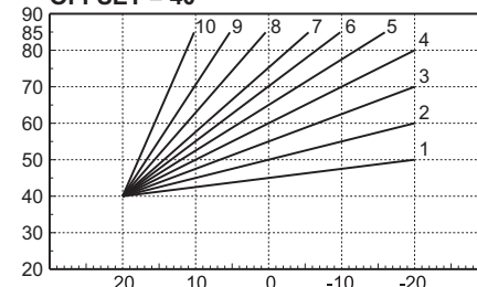
fig. 25- Example of compensation parallel curve offset
