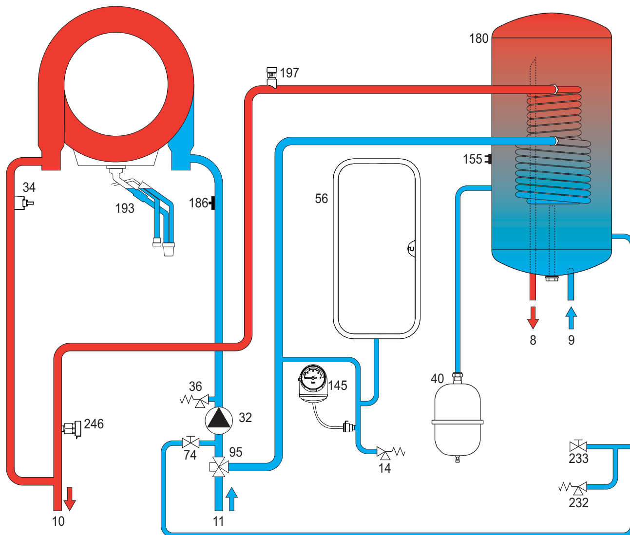
fig. 61- Hydraulic circuit
