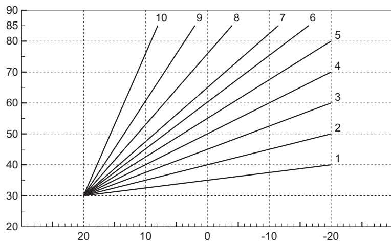
fig. 24- Compensation curves
