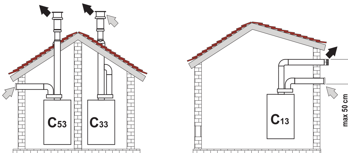
fig. 34- Examples of connection with separate pipes
